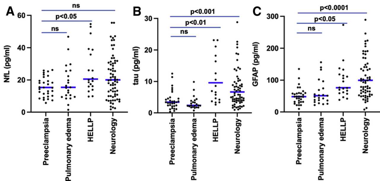
FIGURE 2 Differences between women with different phenotypes of preeclampsia
